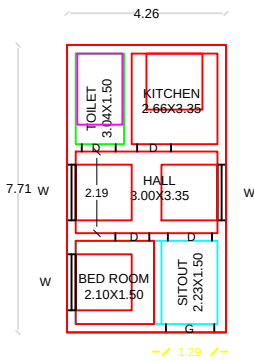
PROPOSED GF PLAN
