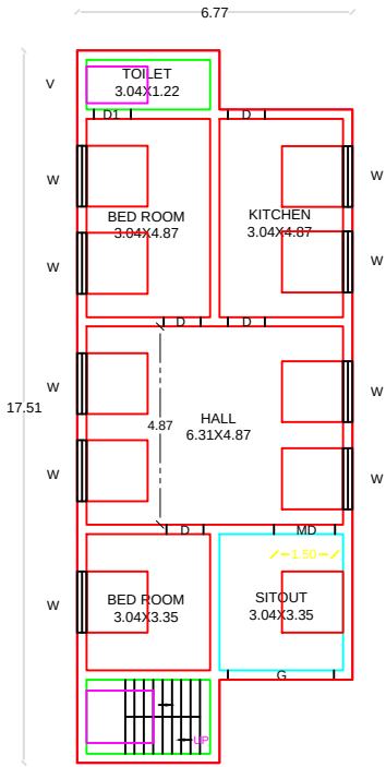
PROPOSED GF PLAN
