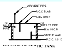
SECTION ON SEPTIC TANK
