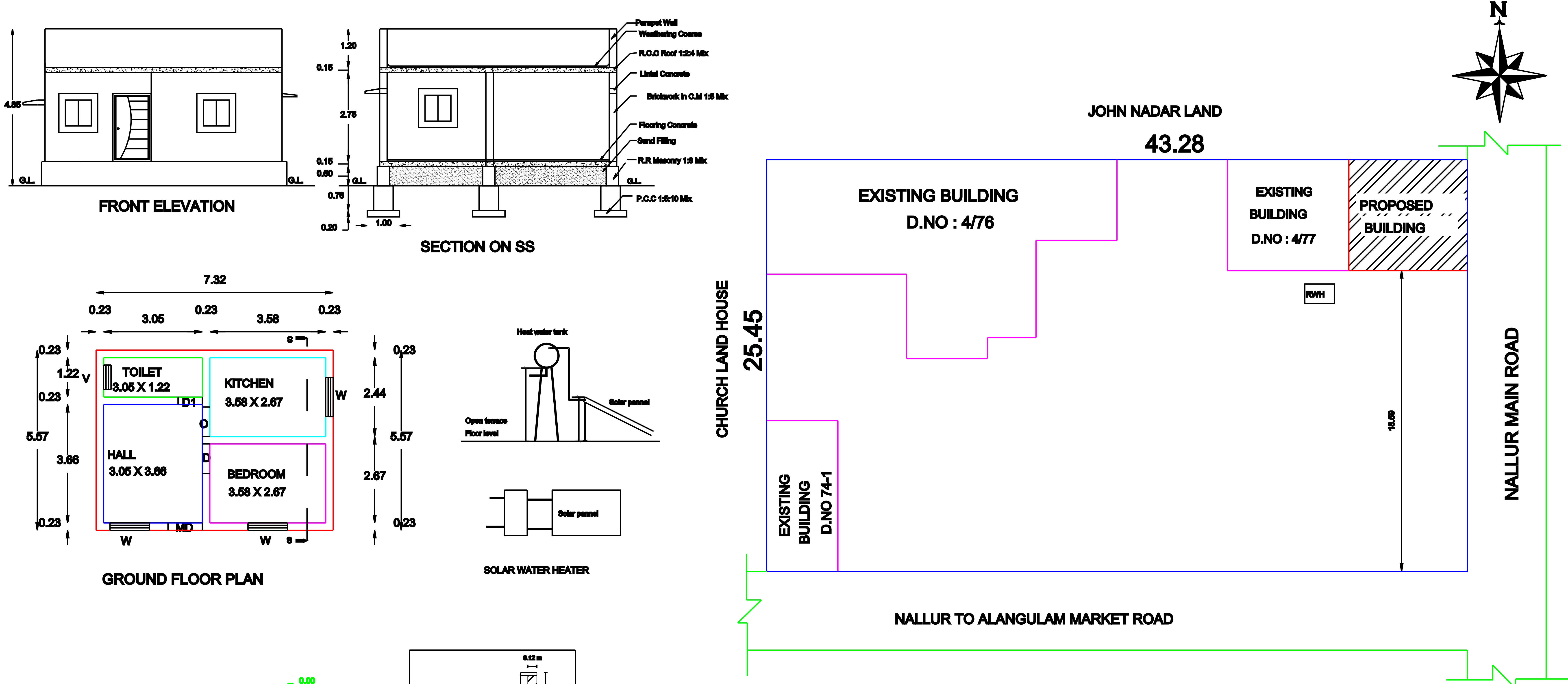
SITE PLAN ( SCALE:- 1:200 )
