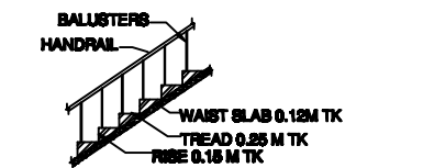
STAIRCASE DETAILS
