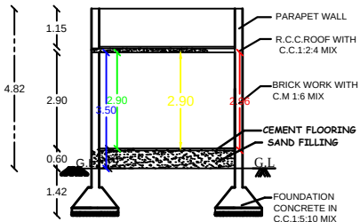
SECTION ON "AB"
