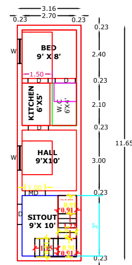
EXT GROUND FLOOR RESIDENTIAL PLAN
