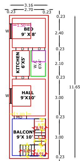
PRO FIRST FLOOR RESIDENTIAL PLAN
