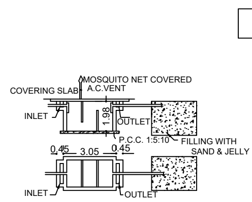
SEPTIC TANK & TRENCH U TRAP PROVISION
