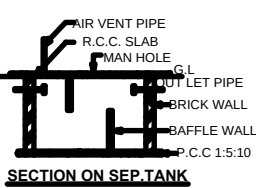
SECTION ON SEP.TANK
