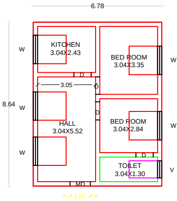
PROPOSED GF PLAN
