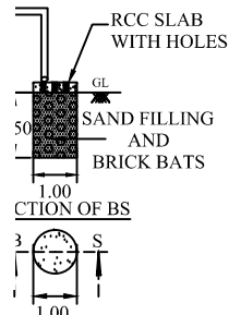
PLAN OF RAINWATER HARVEST TANK
