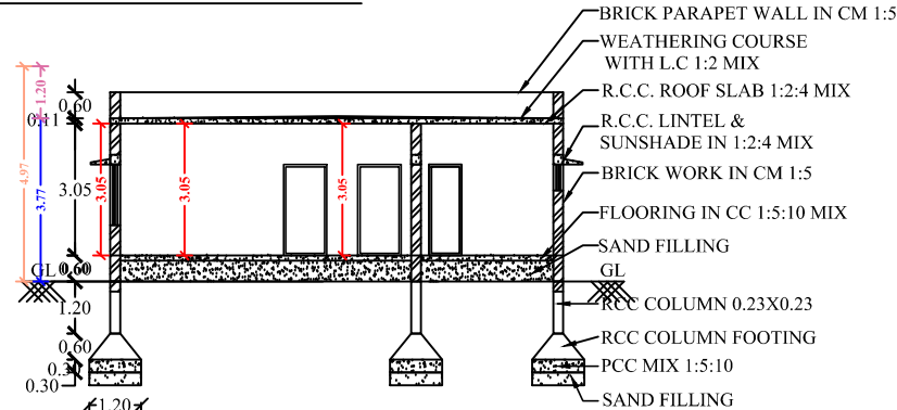
SECTION OF "AB"
