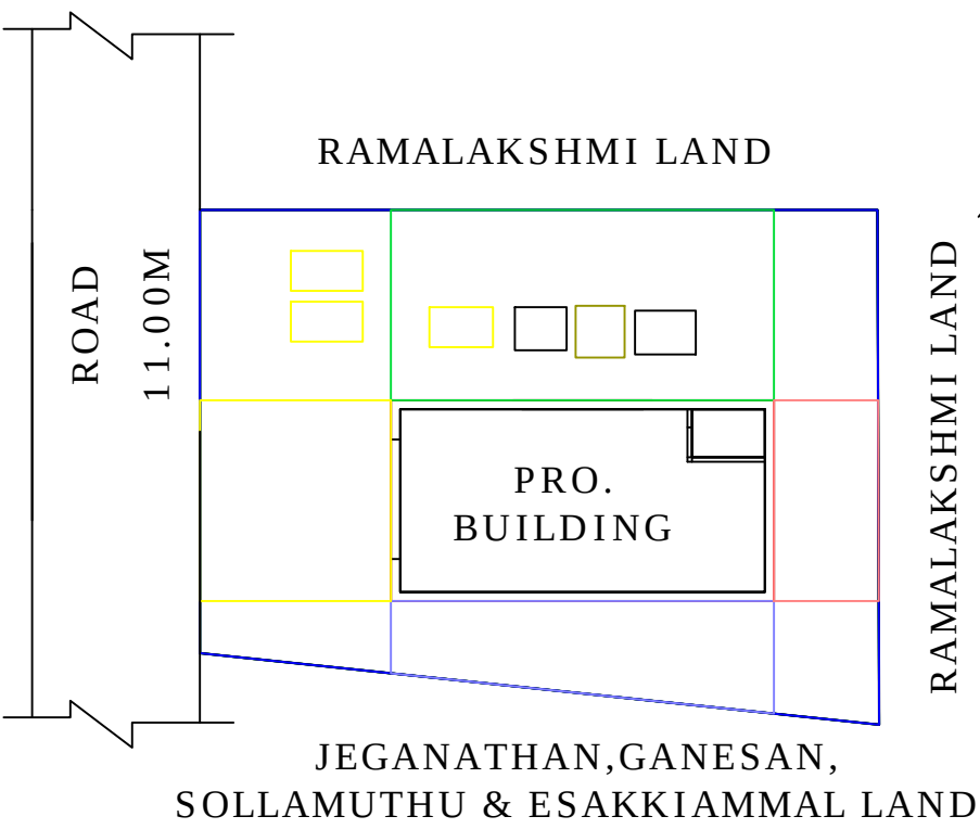
SITE PLAN
