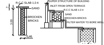
PERCOLATION PIT
