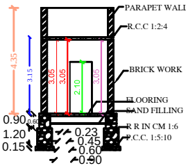
SECTION AB
