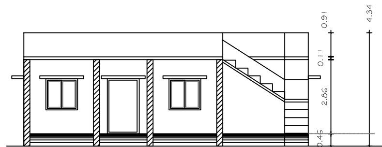
SECTION "A-B"
