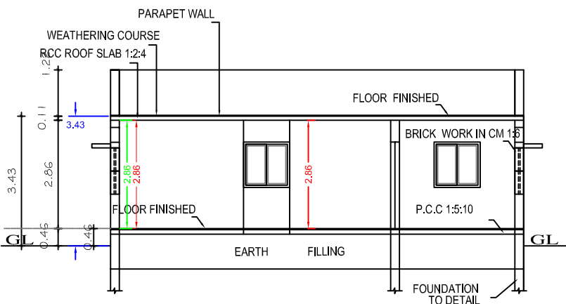
SECTION "A-B"
