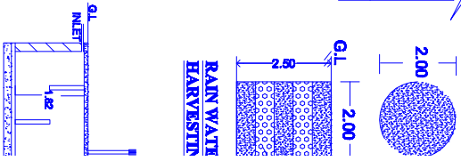
COLUMN DETAILS
