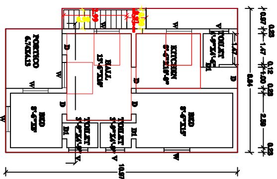
G.F. PLAN
