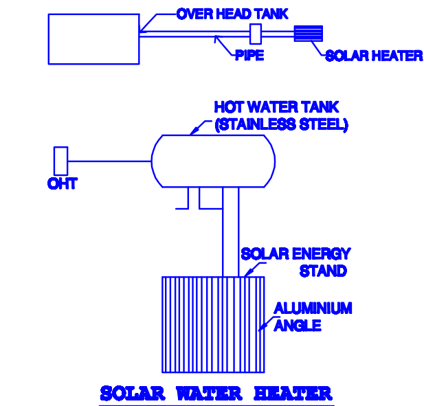
SOLAR WATER HEATER
