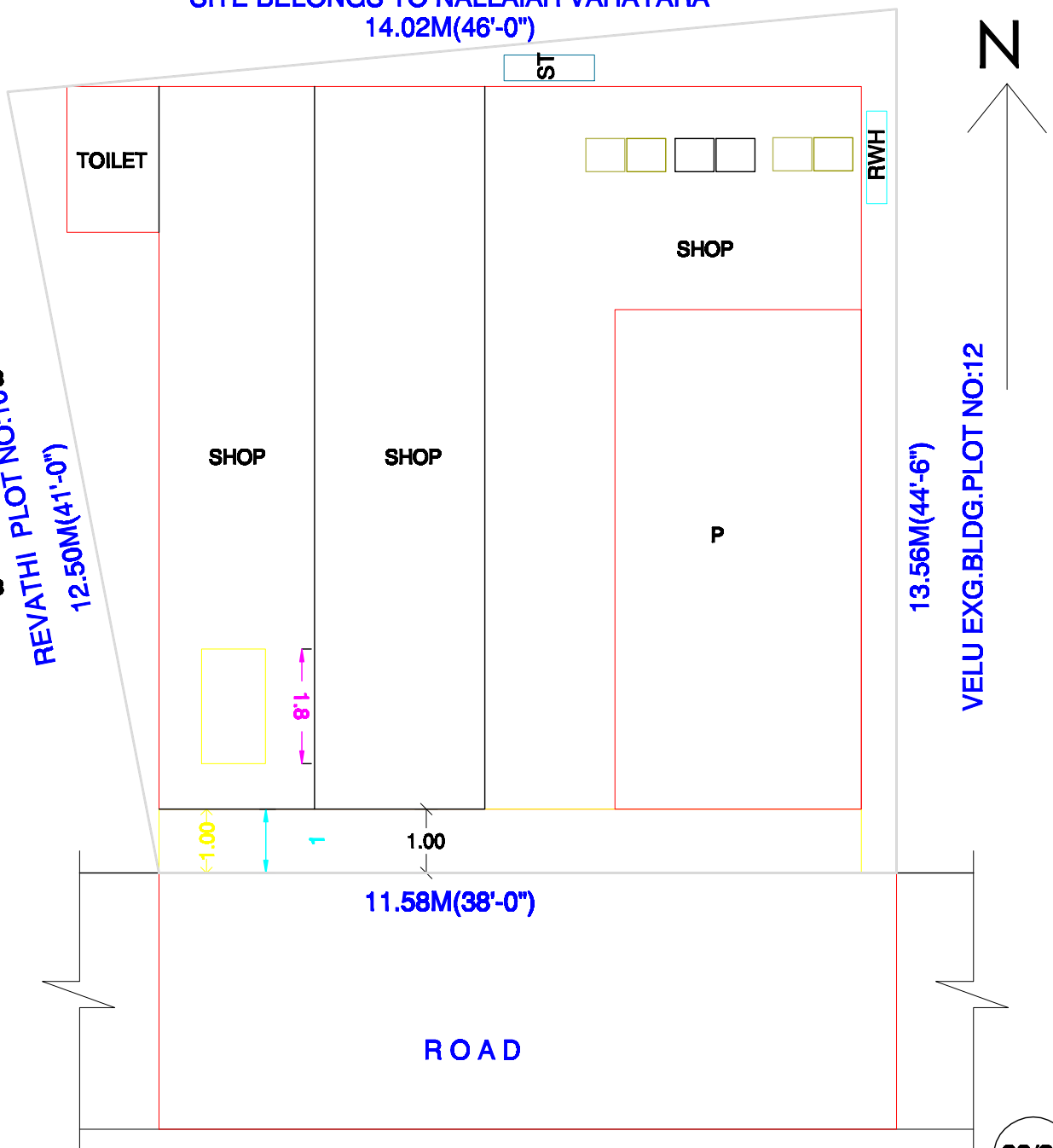
SEPTIC TANK & TRENCH U TRAP PROVISION
