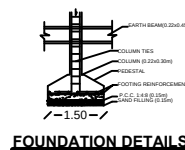
FOUNDATION DETAILS
