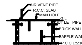
SECTION ON SEP.TANK
