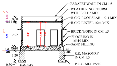
SECTION OF "AB"
