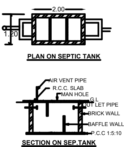
SECTION ON SEP.TANK
