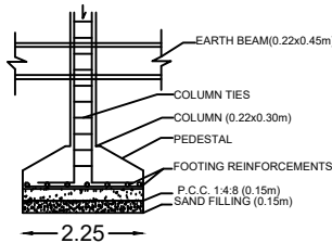
FOUNDATION DETAILS
