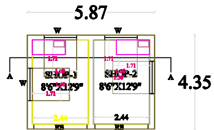
SHOP-1 SHOP-2 GROUND FLOOR PLAN
