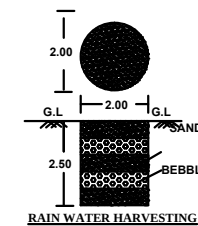
RAIN WATER HARVESTING
