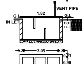
SEPTICTANK DETAILS
