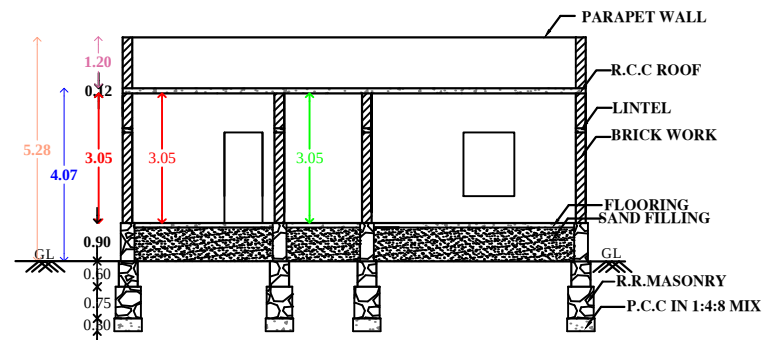
"SECTION "AB"
