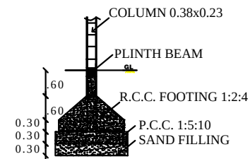
COLUMN DETAILS
