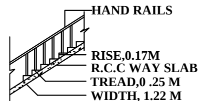
SECTION ON STAIR
