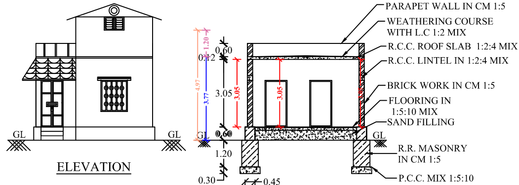
SECTION OF "AB"
