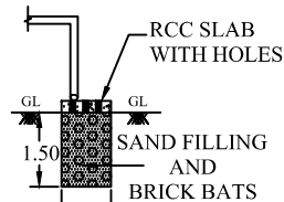
SECTION OF BS
