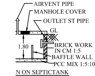
SECTION OF BS
