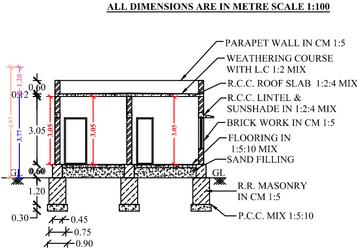
SECTION OF "AB"
