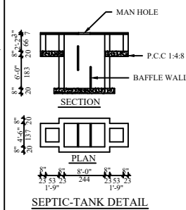
SEPTIC-TANK DETAIL
