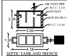
SEPTIC TANK AND TRENCH
