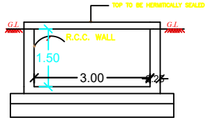
RWH SECTION
