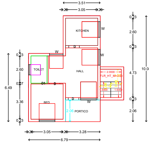
G.FLOOR PLAN
