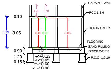
SECTION AB
