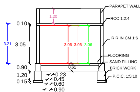
SECTION AB
