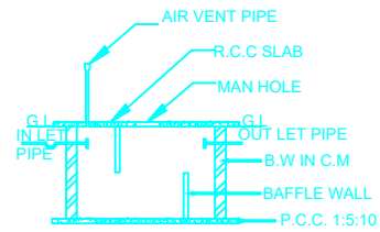
SECTION ON SEPTIC TANK
