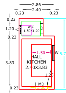
PRO GROUND FLOOR RESIDENTIAL PLAN
