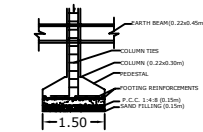
FOUNDATION DETAILS
