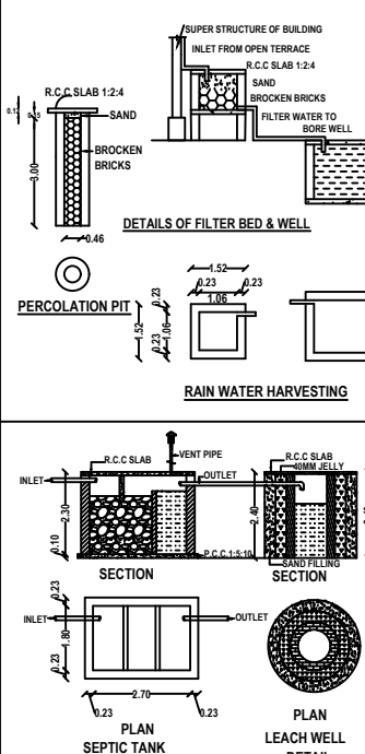
RAIN WATER HARVESTING
