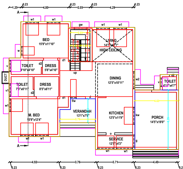
PLAN - GROUND FLOOR RESIDENCE
