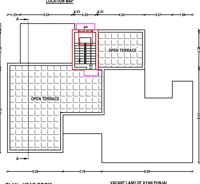
PLAN - HEAD ROOM RESIDENCE
