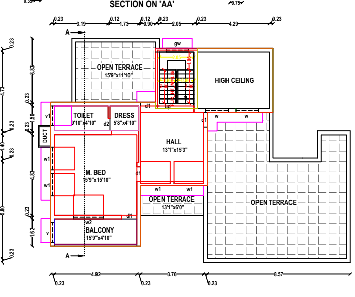
PLAN - FIRST FLOOR RESIDENCE
