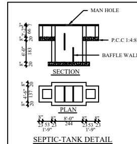
SEPTIC-TANK DETAIL
