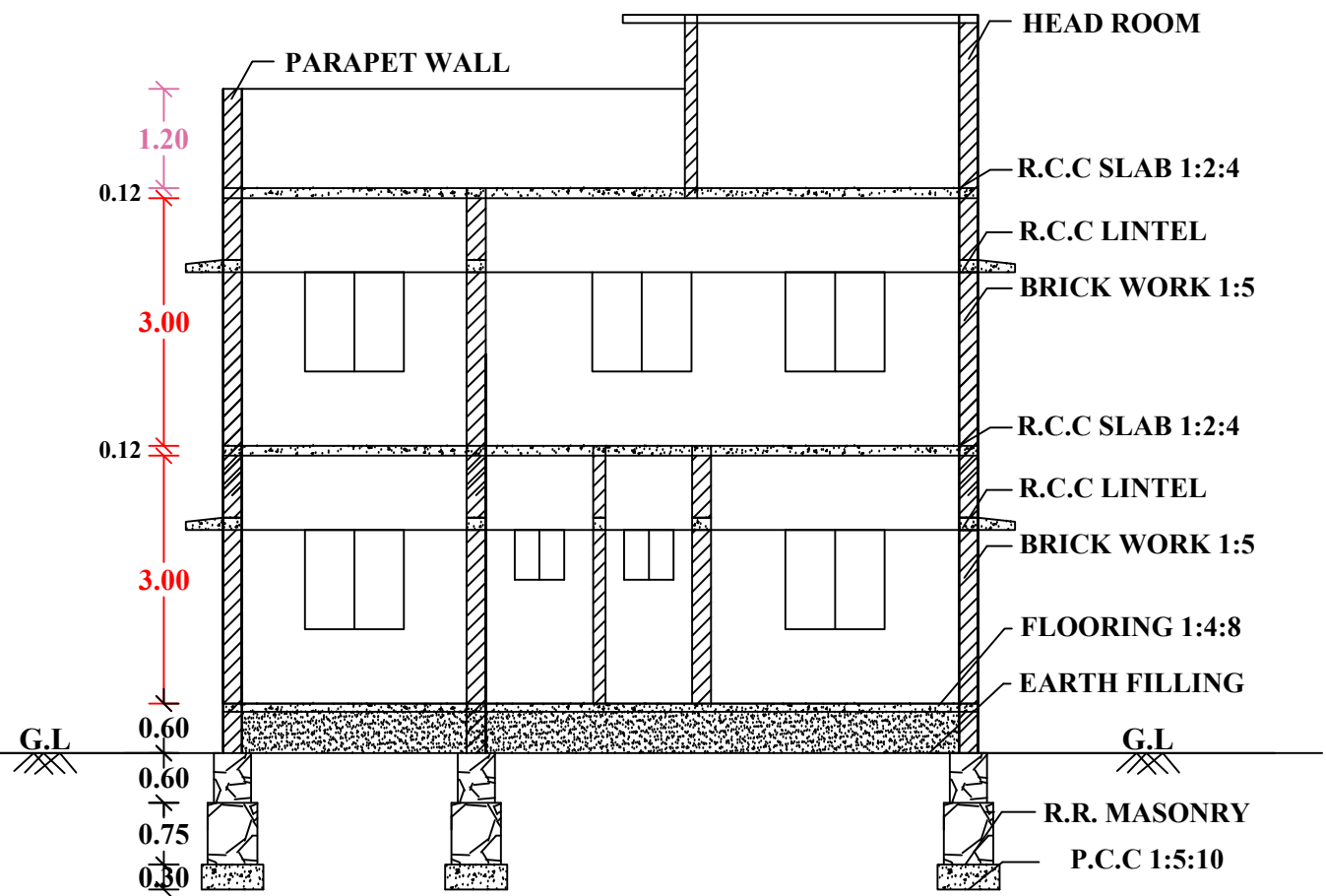
"SECTION "AB"
