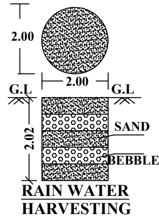
RAIN WATER HARVESTING
