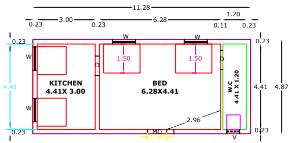
PRO GROUND FLOOR RESIDENTIAL PLAN
