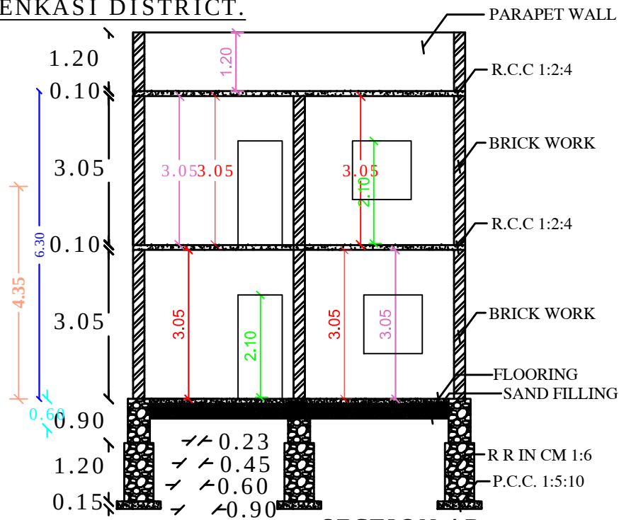
SECTION AB
