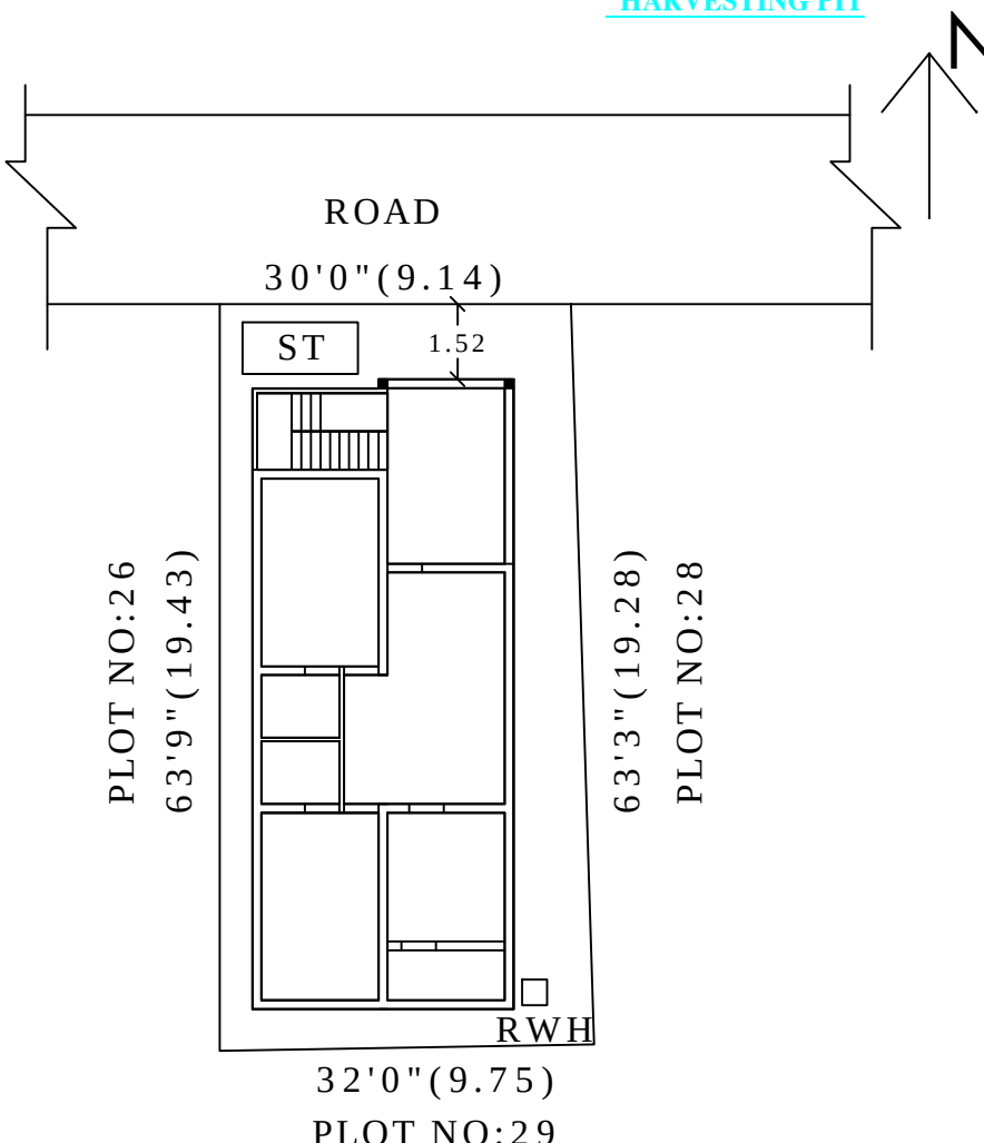
SITE PLAN
