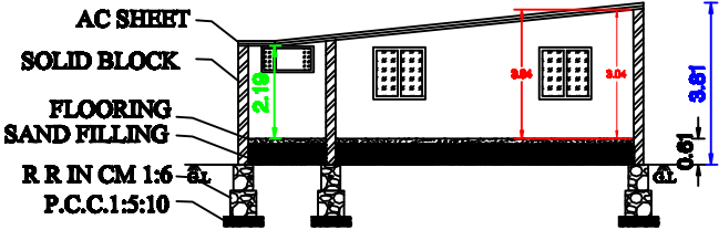
SECTION AB
