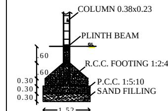
COLUMN DETAILS
