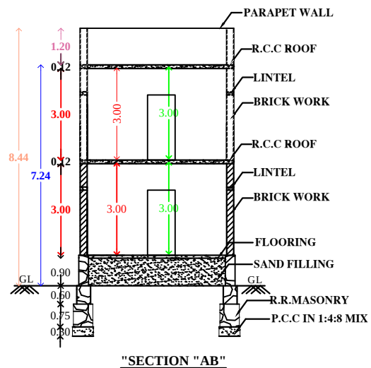
"SECTION "AB"
