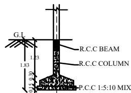
SECTION OF FOOTING
