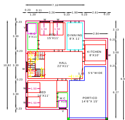
PRO GROUND FLOOR RESIDENTIAL PLAN
