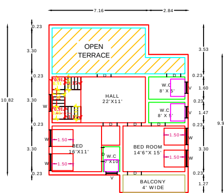
PRO FIRST FLOOR RESIDENTIAL PLAN
