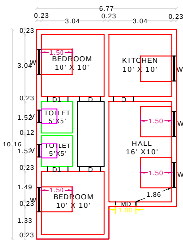
GROUND FLOOR RESIDENTIAL PLAN
