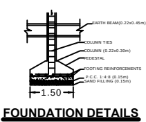
FOUNDATION DETAILS
