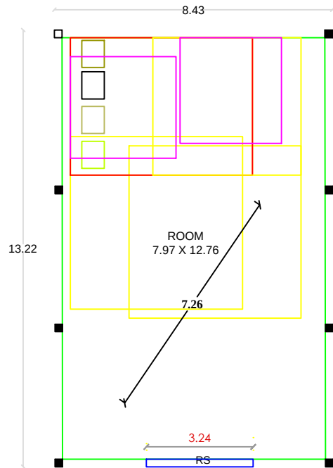
PLAN
