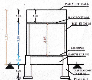
SECTION AB
