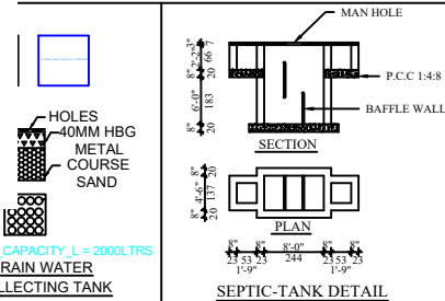
SEPTIC-TANK DETAIL
