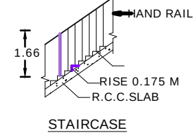
STAIRCASE
