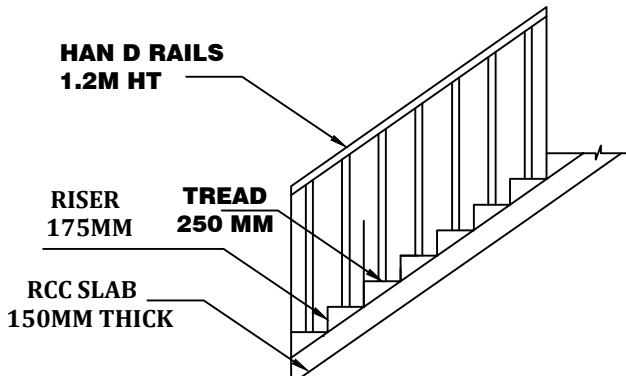
STAIRCASE DETAILS SCALE 1:50
