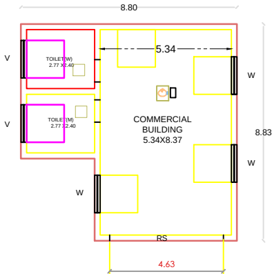
PROPOSED GF PLAN
