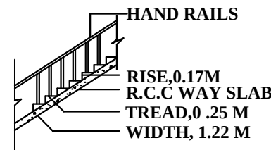
SECTION ON STAIR
