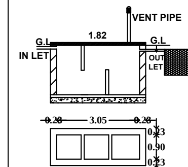
SEPTICTANK DETAILS
