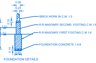
FOUNDATION DETAILS
