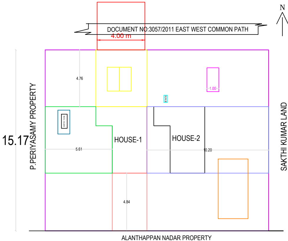
18.71 SITE PLAN
