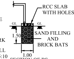
SECTION OF BS
