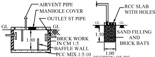
SECTION ON SEPTICTANK
